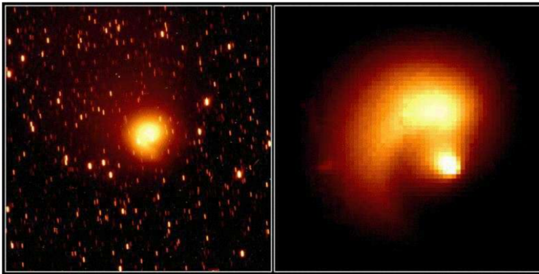
FIRST PICTURES OF HALE BOPP FROM THE HUBBEL SPACE TELESCOPE CLEARLY SHOWING ITS ORBITING COMPANIONS
