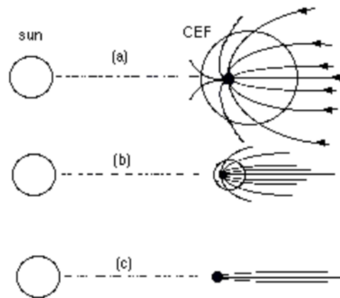
MY 1970s DRAWING OF COMETS MY PLASMA DISCHARGE COMET MODEL
