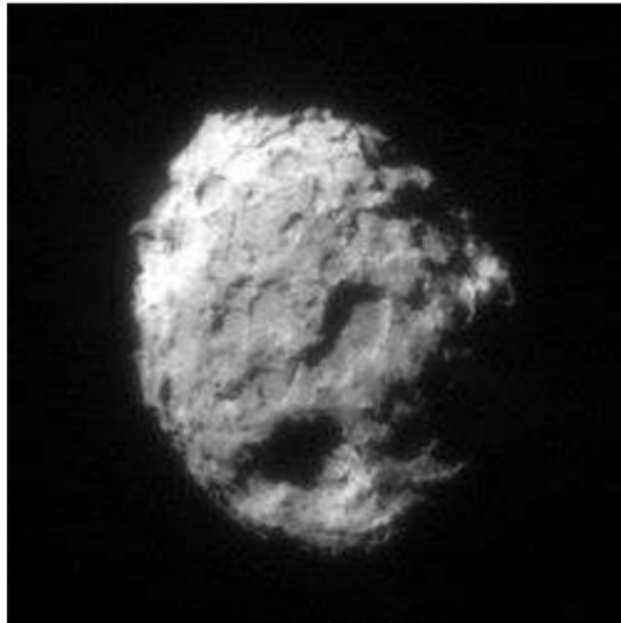
COMET WILD 2 – STARDUST MISSION IT HAS NO SURFACE ICE – HARD SOLID CRATERED HOT ROCK SO WHY DO THEY STILL REPEAT THAT THIS IS A DIRTY SNOWBALL ???
