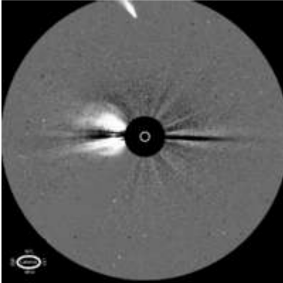
SOHO IMAGE OF COMET IGNITING CORONAL MASS EJECTION PROVING ALSO MY THEORY THAT COMETS INTERACT WITH THE SUN
