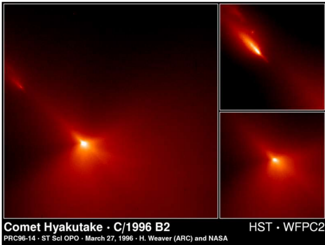
COMET HYAKUTAKE AT CLOSEST APPROACH TO EARTH – MARCH 1996
