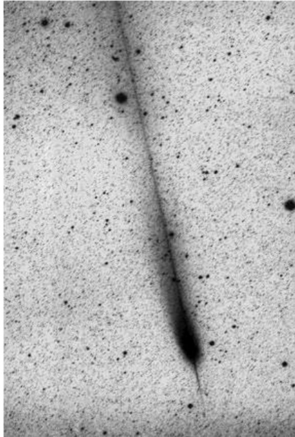
COMET HALE BOPP WITH SUNWARD ELECTRICAL SPIKE AT CLOSEST APPROACH TO THE SUN AS IT CROSSES THE ECLIPTIC
