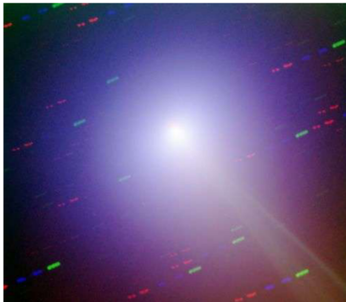
COMET LINEAR BRILLIANT COMET NOT JUST REFLECTED LIGHT
