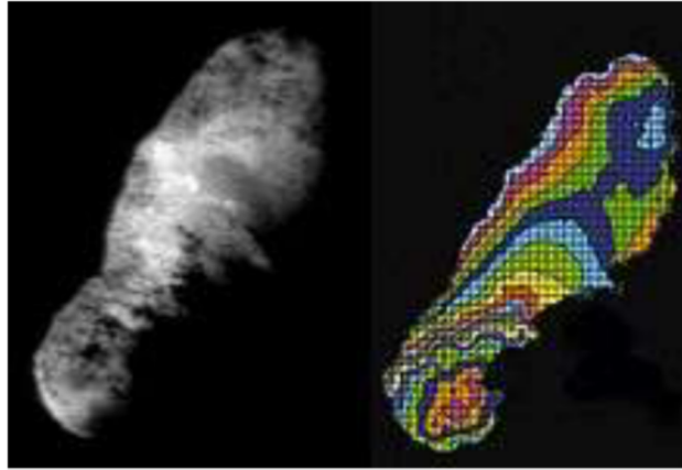
COMET BORRELLY HAS NO SURFACE ICE
